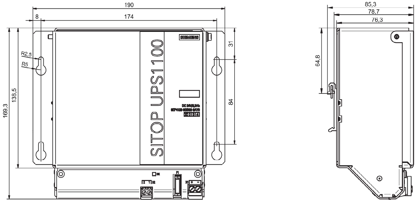
Figure 2-25 6EP4133-0GB00-0AY0 dimensioned drawing
