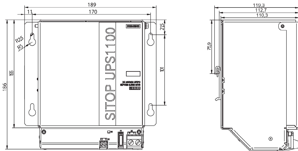
Figure 2-26 Dimension drawing 6EP4133-0JB00-0AY0
