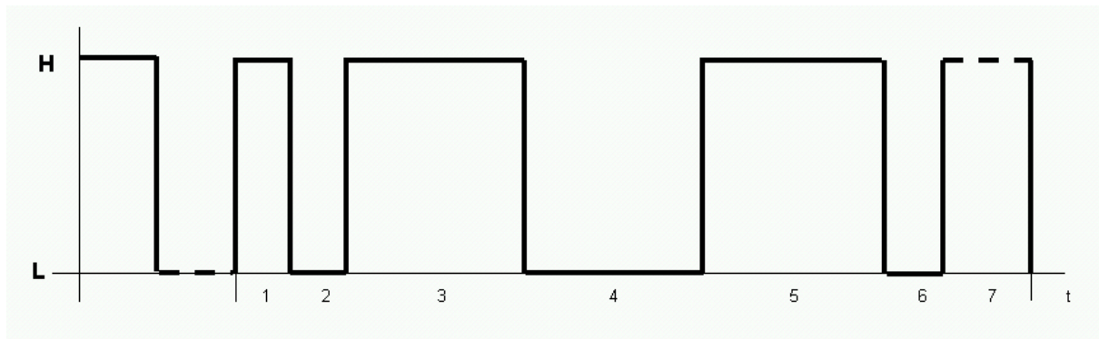
Diagram 1: Remote signal to Pin 7 (Pin 4 in case of 25-pole plug/socket) of the serial interface
